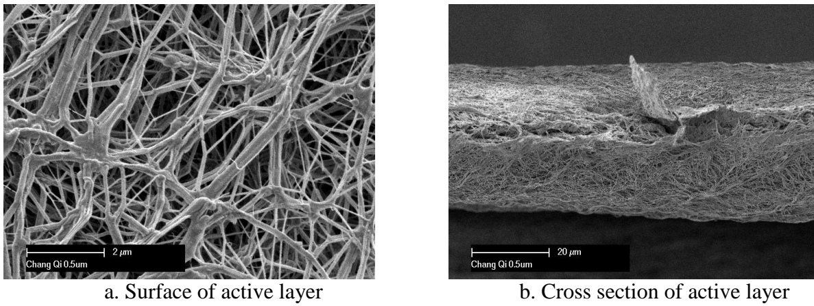
Fig. 5 Images for membrane structure
