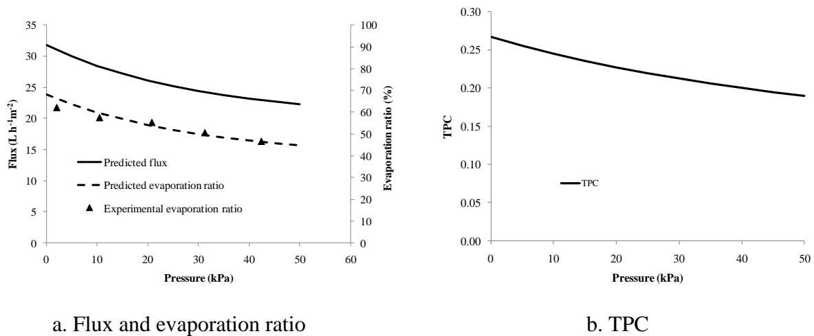
Fig. 11 Influence of the pressure ( L_{mem} = 131 mm, T_{fi} = 60^\circ\text{C} , T_{pi} = 20^\circ\text{C} , v_f = v_p = 0.0945 m/s)
